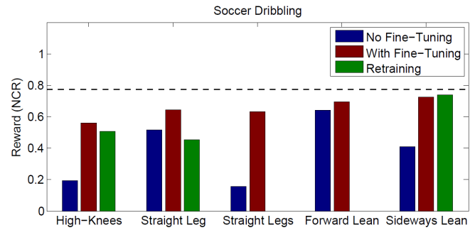
Fig. 13. Performance using different LLC's for soccer dribbling with and without HLC fine-tuning, and retraining.
