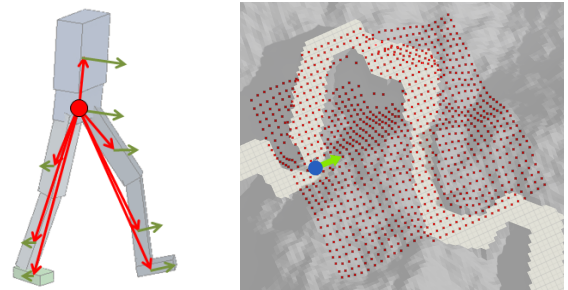
Fig. 3. left: The character state features consist of the positions of each link relative to the root ( red arrows ), their rotations, linear velocities ( green arrows ), and angular velocities. right: The terrain features consist of a 2D heightmap of the terrain sampled on a regular grid. All heights are expressed relative to height of the ground immediately under the root of the character. The heightmap has a resolution of 32x32 and occupies an area of approximately 11x11m.
